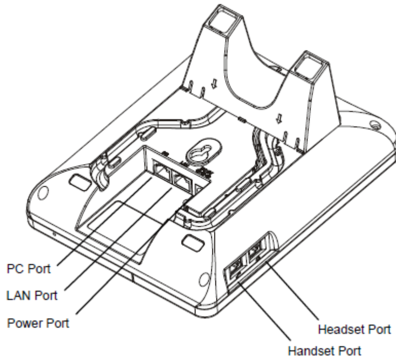
Figure 1: GXP1160/GXP1165 Ports
