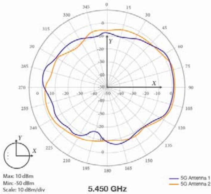
Horizontal or Azimuth (Top View)
